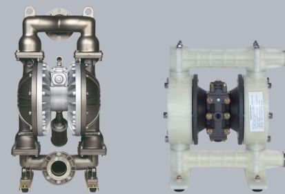
HIGH PERFORMANCE AIR-POWERED DOUBLE DIAPHRAGM Pumps
